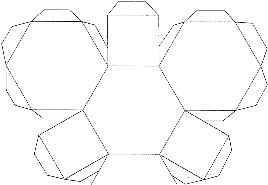
Truncated Octahedron
